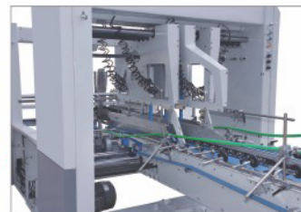
Pre-folding Part
