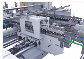
Alignment Part
