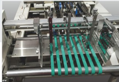
Feeding
